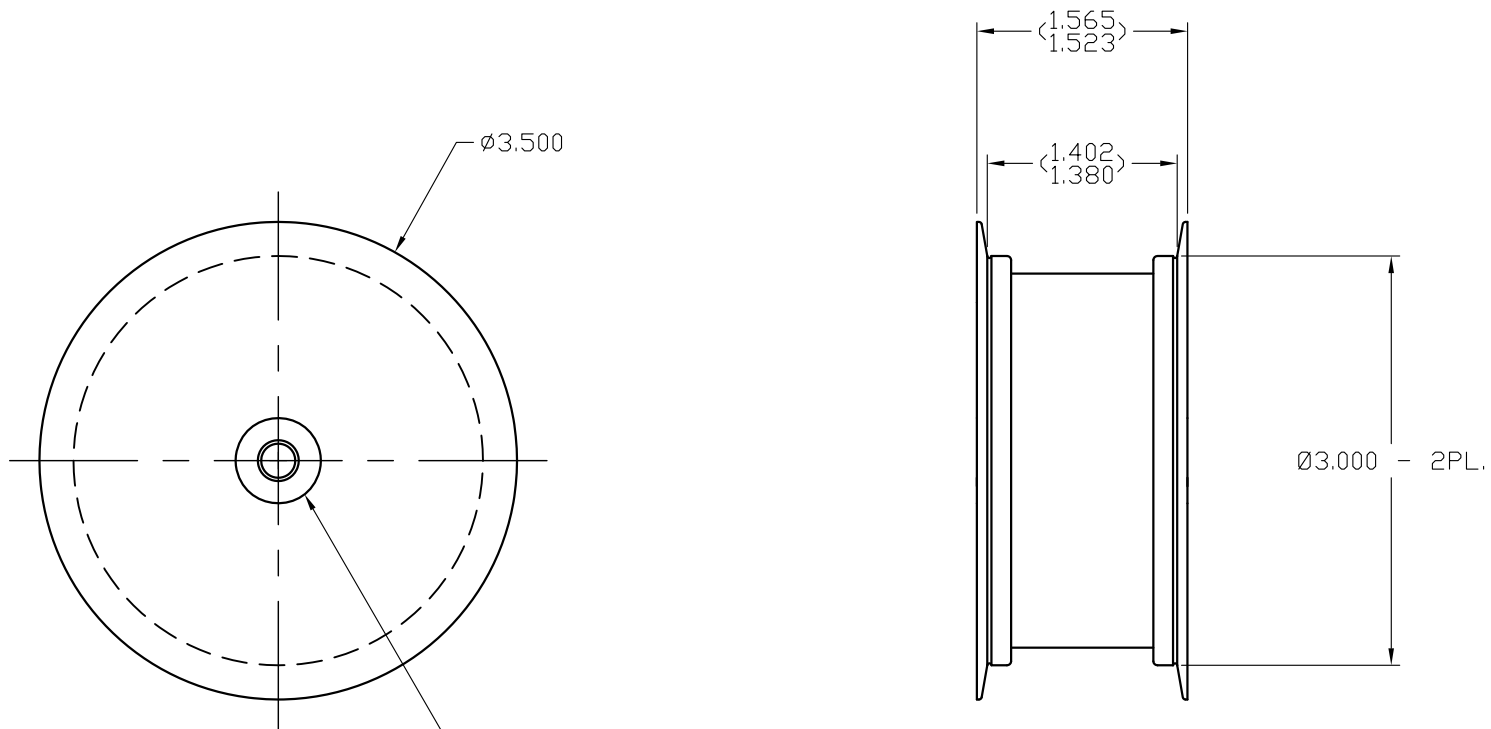
PP1002 BEARING - RADIAL, 1/4" ID (CRES) - 2PL.
