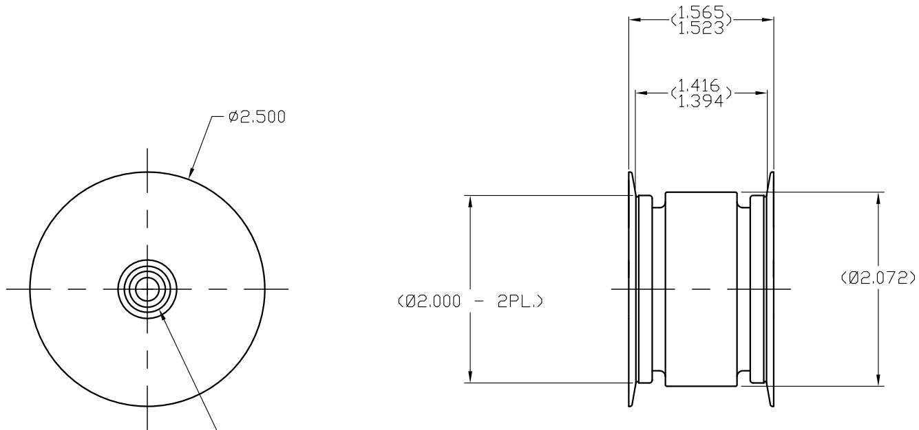
PP1002 BEARING - RADIAL, 1/4" ID (CRES) - 2PL.
